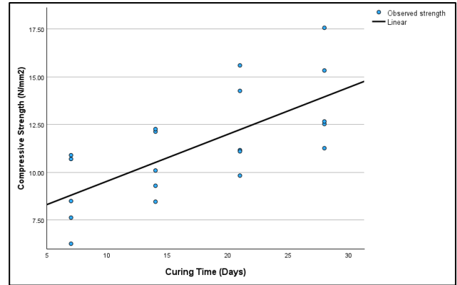
Figure 6. Linear regression curve estimation of compressive strength vs curing time
