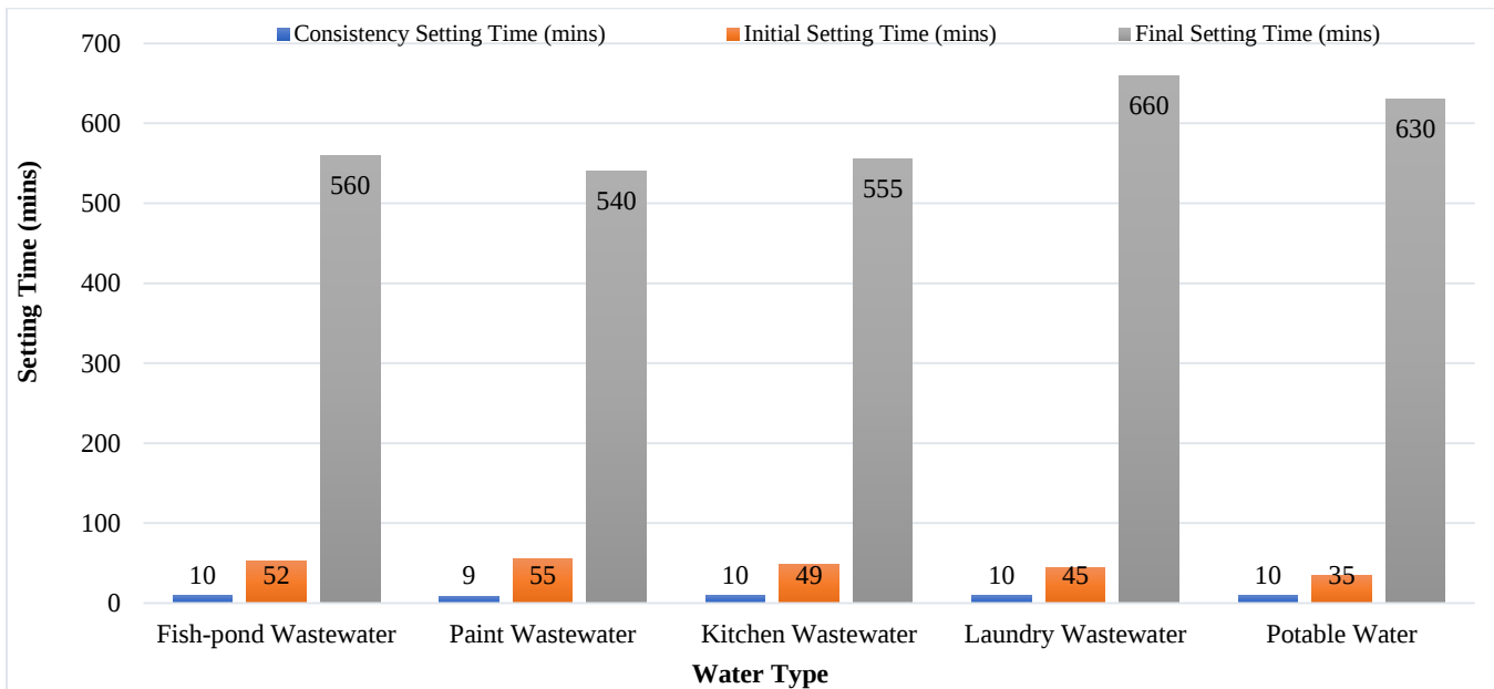
Figure 2. Chart of setting times of cement vs water types
